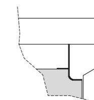
GOLA MOD. PLANA PLANA MODEL GRIP PROFILE
